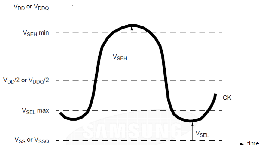
Figure 3. Single-ended requirement for differential signals
