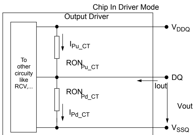
Figure 16. Output Driver
