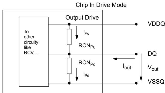
Figure 15. Output driver
