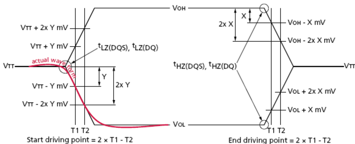
Data Out measurement reference points
