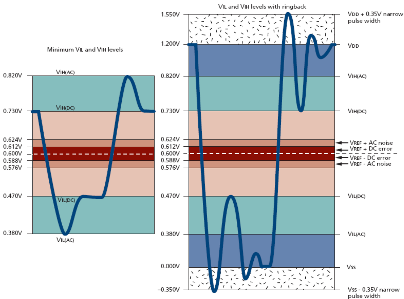
LPDDR2 1066 Input Signal
