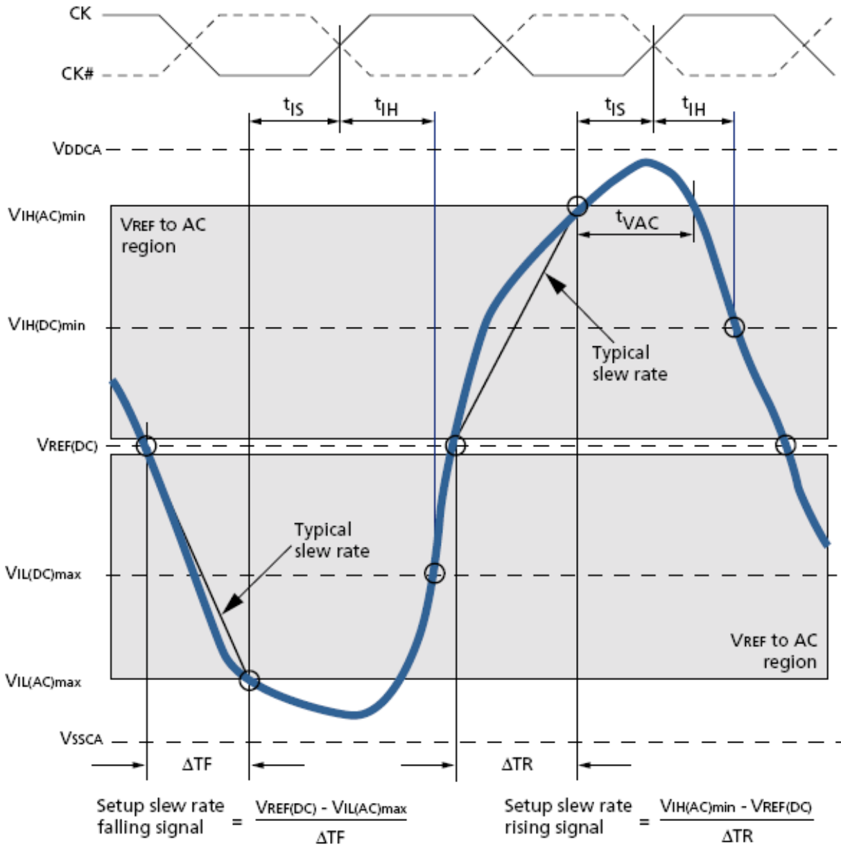
Illustration of nominal slew rate and tvac for setup time ts for CA and \overline{CS} with respect to clock
