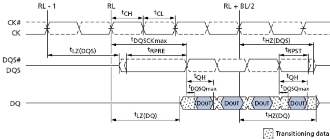
Data output (Read) timing (tDQSKmax)
