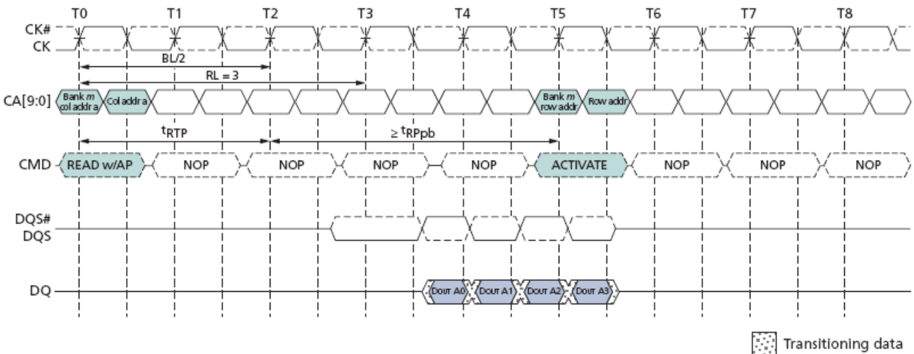
Burst Read with Auto-Precharge: RL=3, BL=4, RU('RTP(\text{min})/CK)=2
